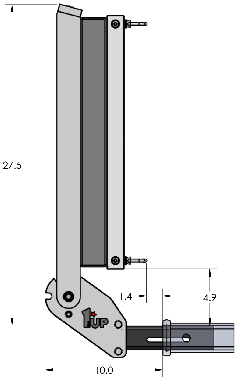
STORAGE POSITION
