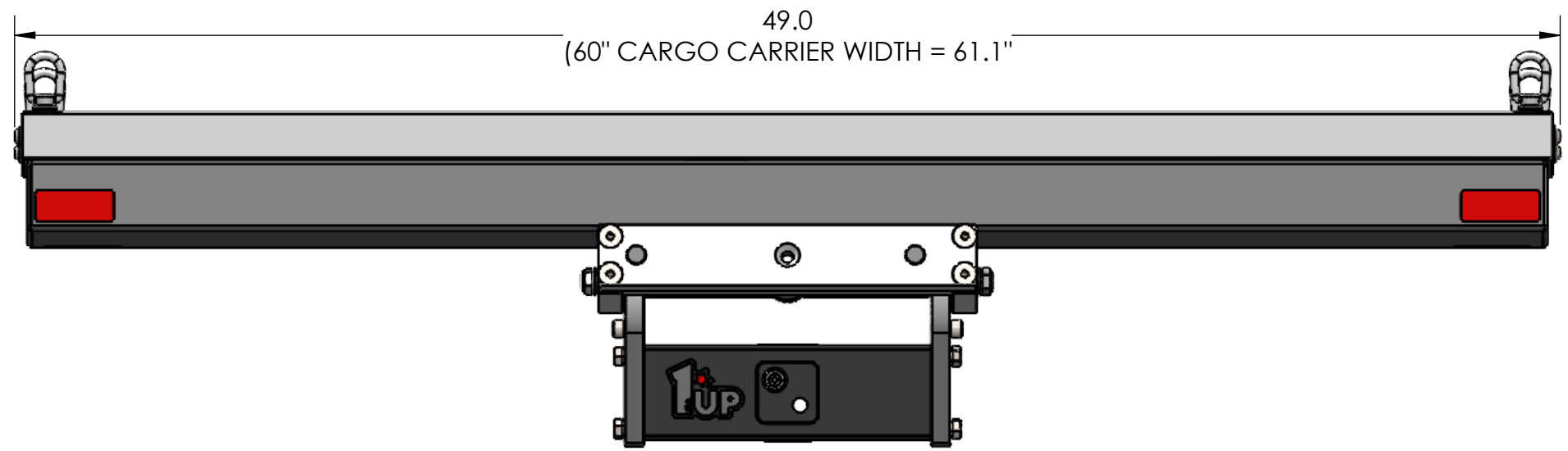
OVERALL WIDTH
