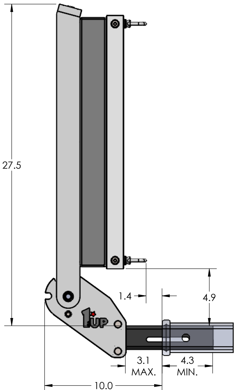
BASE RACK
